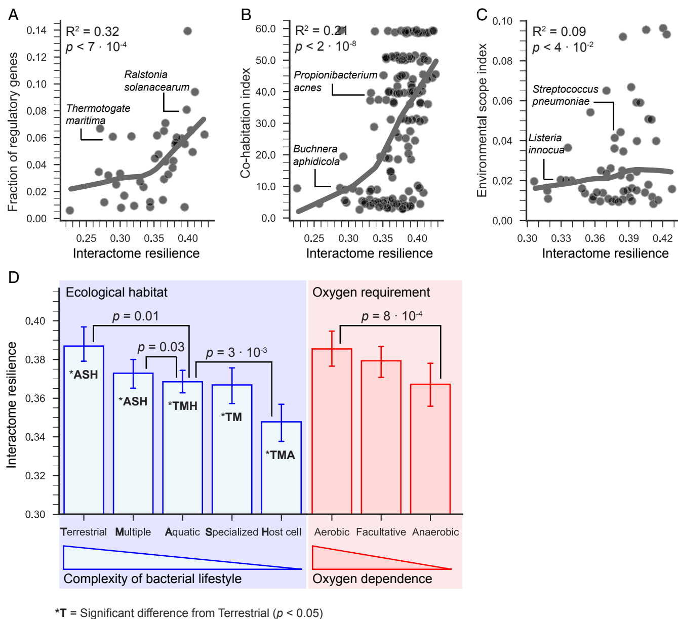
Fig. 2. Bacteria with more resilient interactomes survive in more complex, variable, and competitive environments. We use ecological information for 287 bacterial species (32) to examine the relationship between species' interactome resilience and their ecology ( SI Appendix , section S4). (A) Interactome resilience positively correlates with the fraction of regulatory genes in bacteria, an established indicator of environmental variability of species' habitats (32) ( R^2 = 0.32 ). (B and C) For environmental viability of a species, we use a cohabitation index that records how many organisms populate each environment in which the species is viable (i.e., the level of competition in each viable environment) and an environmental scope index that records a fraction of the environments in which the species is viable (i.e., species' environmental diversity) (32). The resilience of the interactome positively correlates with the level of cohabitation encountered by bacteria ( R^2 = 0.21 ), and bacteria with resilient interactomes tend to thrive in highly diverse environments ( R^2 = 0.09 ). (D) Terrestrial bacteria have the most resilient interactomes ( P = 7 \cdot 10^{-3} ), and host-associated bacteria have the least resilient interactomes ( P = 4 \cdot 10^{-6} ). In bacteria, interactome resilience is indicative of oxygen dependence. Aerobic bacteria have the most resilient interactomes ( P = 8 \cdot 10^{-4} ), followed by facultative and the anaerobic bacteria. Error bars indicate 95% bootstrap confidence interval; P values denote the significance of the difference of the means according to a Mann-Whitney U test.
