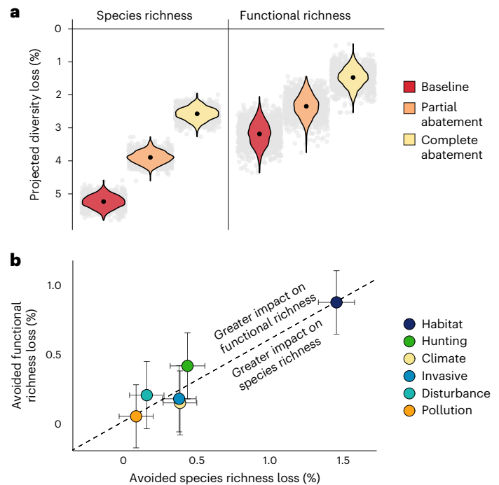
Fig. 1 | Projected loss of avian diversity in the next 100 years. a , Loss in species richness and functional richness under three scenarios: baseline extinction, partial abatement of all drivers of extinction and complete abatement of all drivers of extinction. Black points show mean loss across 1,000 iterations for each scenario, with variation in those points shown by their distribution (violin plots) and the individual values (grey dots). b , Diversity loss avoided under driver-specific complete abatement of six major drivers of extinction (circles represent the mean; error bars, 0.5 s.d.). Note that in some iterations, loss avoided could be negative, as more diversity was lost with driver-specific abatement than under the baseline scenario. The dotted diagonal line shows mean functional richness loss per species richness loss under complete abatement of all threats. Drivers above this line show greater avoidance of functional richness loss per species richness loss avoided relative to the mean across all drivers of extinction. Hunting, hunting and collection; climate, climate change and severe weather; invasive, invasive species, genes and disease; disturbance, disturbance and accidental mortality. Analyses based on 9,873 species (of which 2,087 species currently listed as Near Threatened or in threatened categories were modelled and could have reduced extinction risk in the abatement scenarios). A total of 1,000 iterations were run for each extinction scenario.
