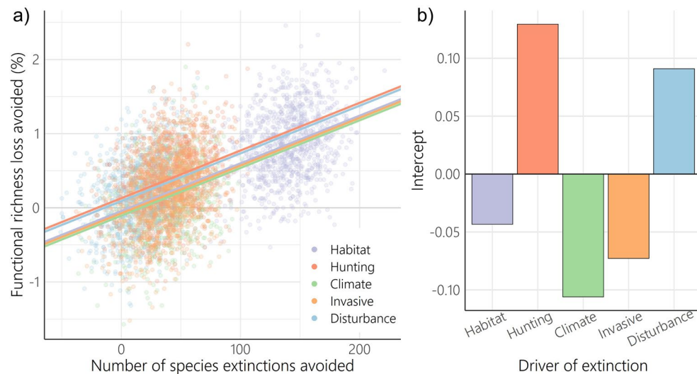
Extended Data Fig. 6 | Abatement of hunting and collection, and disturbance and accidental mortality provides disproportionate benefits for functional richness. a , Number of species extinctions avoided under driver-specific complete abatement against functional richness loss avoided (% of functional richness of full assemblage) as described by a linear mixed effects model including number of species extinctions avoided and driver of extinction as fixed effects, and iteration number as a random effect. b , Intercepts of linear mixed effect model of number of species extinctions avoided against functional
